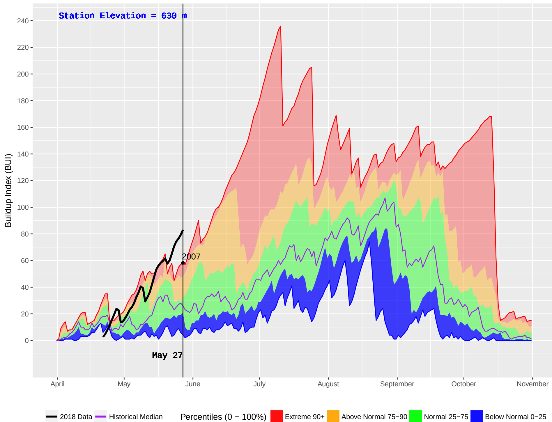
ANDERSON CREEK (977) : Historical (2007–2016) and Current (2018) Noon Buildup Index (BUI)
